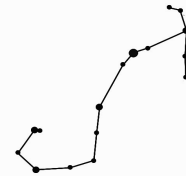
Scorpius, the Scorpion
